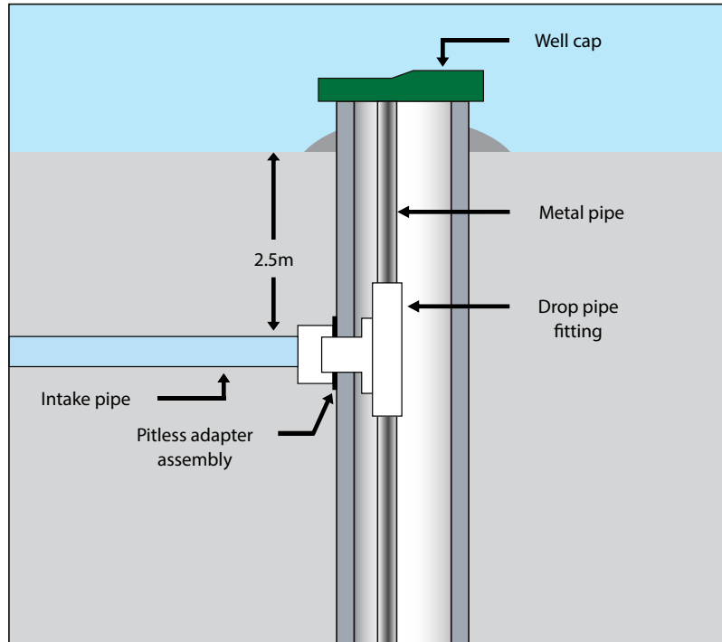
Figure 8. Example of a pitless adapter.
